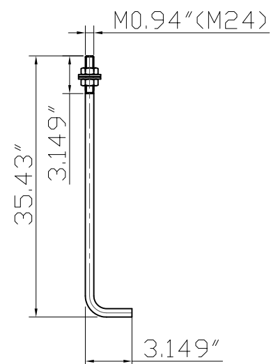
ANCHOR BOLTS 4PCS PER POLE
