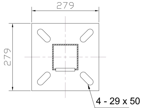
A-A VIEW (3:1)
