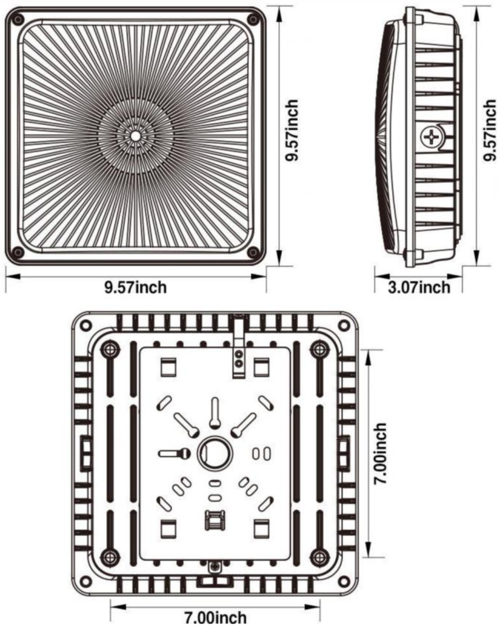
45~70W Drawing
