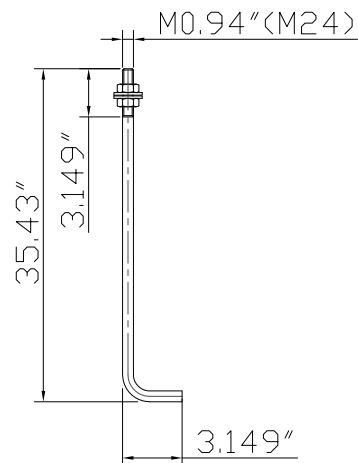
ANCHOR BOLTS 4PCS PER POLE
