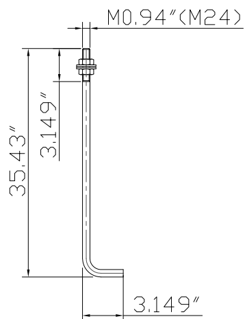
ANCHOR BOLTS 4PCS PER POLE
